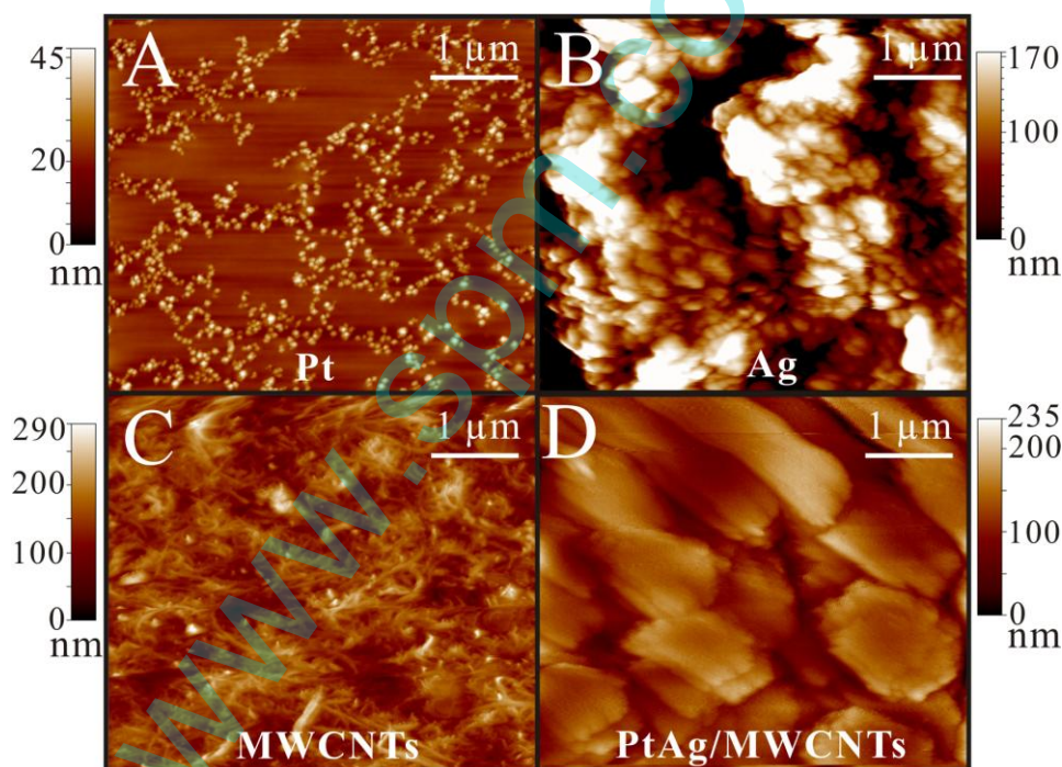
Figure 3. AFM images of (A) Pt, (B) Ag, (C) MWCNTs, and (D) PtAg/MWCNTs coated ITO electrodes.
