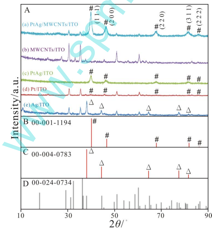
Figure 2. (A) XRD spectra of different modified ITO electrodes. Standard XRD patterns: (B) Pt, (C) Ag, and (D) ITO, respectively.
