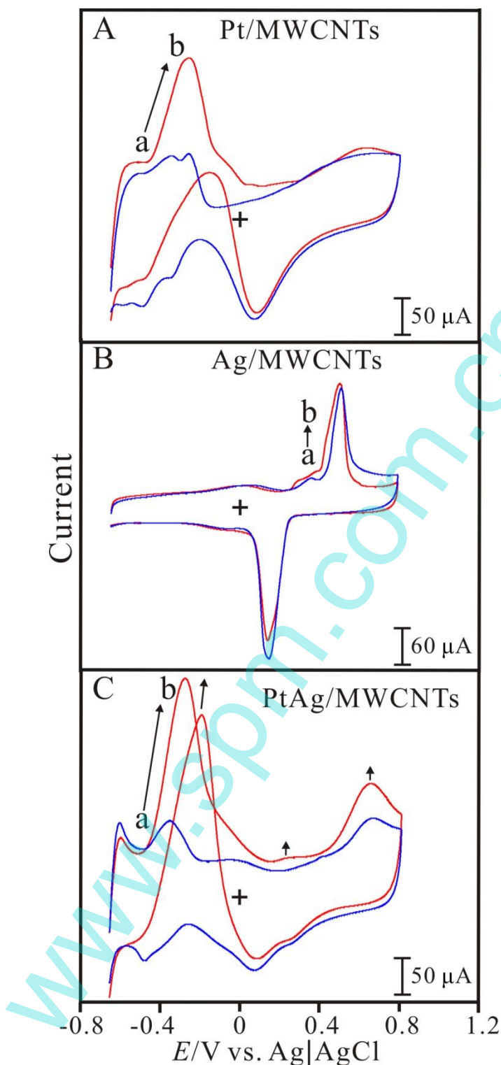
Figure 4. Cyclic voltammograms of (A) Pt/MWCNTs/GCE, (B) Ag/MWCNTs/GCE, (C) PtAg/MWCNTs/GCE examined in the (a) absence and (b) presence of 24 mM glucose (pH 7 PBS). Scan rate = 0.05 \text{ V s}^{-1} .
