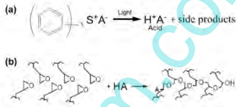
Fig. 4. The detailed reaction yielded by exposing and hard-baking the photosensitive polymer SU-8 2005. (a) Illustration of the UV-induced reaction of SU-8 2005; (b) Illustration of the temperature-induced reaction of SU-8 2005.
