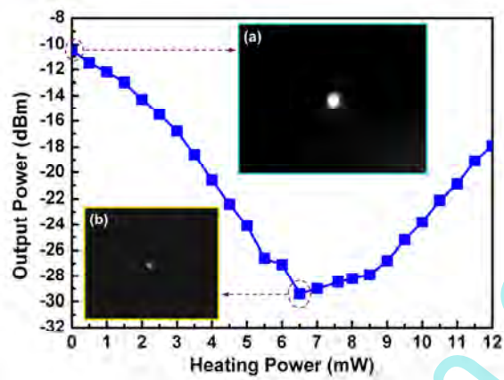
Fig. 8. Measured curve of output power versus heating power. The insets show the near-field guided-mode of the device at 1550 nm wavelength under (a) ON-state and (b) OFF-state.
