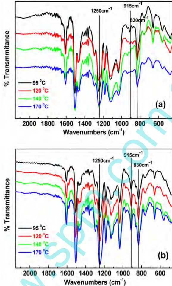
Fig. 5. FTIR spectra of (a) exposed and (b) unexposed SU-8 2005 films at various hard-baking temperatures.
