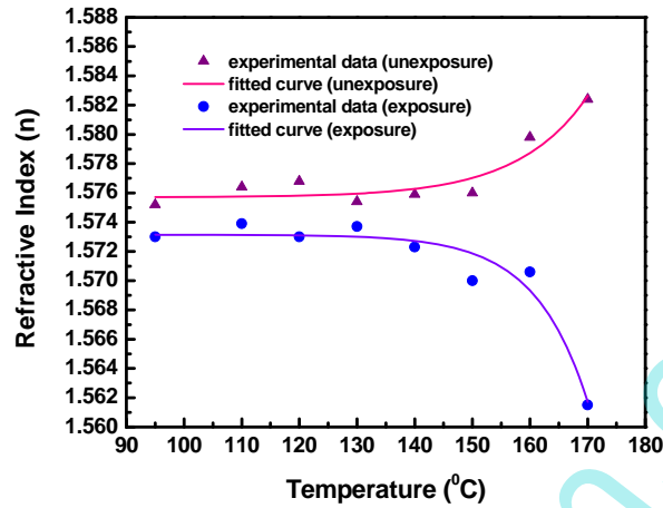
Fig. 3. Curves of refractive indices of the exposed and unexposed films at 1550 nm wavelength versus the hard-baking temperatures.
