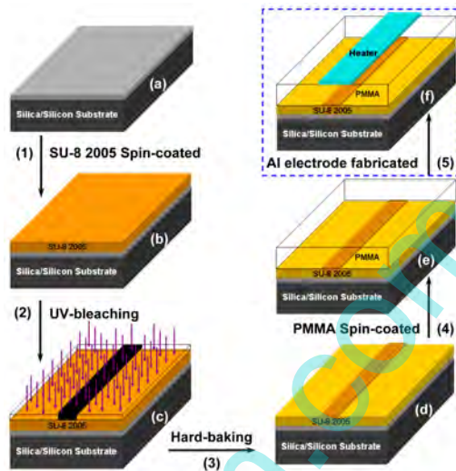
Fig. 6. Fabrication process of waveguide device.
