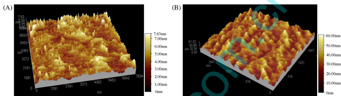
Fig. 4. AFM images of a clean glass surface (A) and a glass surface with a layer of adsorbed sodium alginate in the dry state (B).
